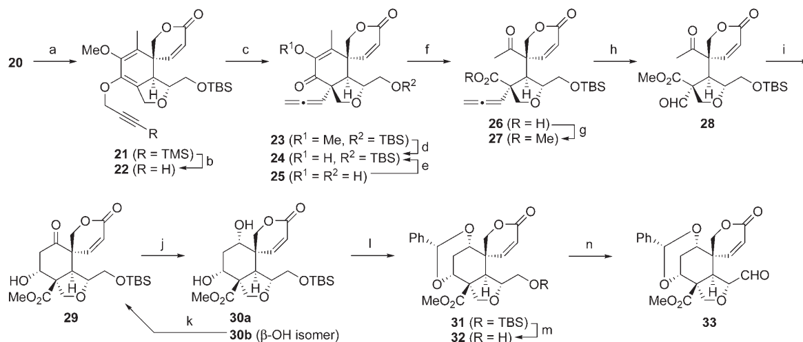
Scheme 5. Construction of the A ring. Reagents and conditions: a) DMF, 120 °C, 66%; b) \text{K}_2\text{CO}_3 , MeOH, RT; c) toluene, reflux, quant. (2 steps); d) \text{BBr}_3 , \text{CH}_2\text{Cl}_2 , 0 °C, 24 % ( 24 ) and 67 % ( 25 ); e) TBSOTf, imidazole, DMF, RT, 87%; f) \text{O}_2 , h\nu , methylene blue, MeOH, 0 °C; g) \text{CH}_2\text{N}_2 , EtOAc, 0 °C, 90 % (2 steps); h) \text{O}_3 , \text{CH}_2\text{Cl}_2 , then \text{Me}_2\text{S} , -78 °C; i) \text{Sn}(\text{OTf})_2 , 4-Å MS, \text{Et}_3\text{N} , \text{CH}_2\text{Cl}_2 , RT, 74 % (2 steps); j) t\text{BuNH}_2\cdot\text{BH}_3 , \text{CH}_2\text{Cl}_2 , RT, 43 % ( 30a ) and 35 % ( 30b ); k) DMP, \text{NaHCO}_3 , \text{CH}_2\text{Cl}_2 , 0 °C, 74%; l) \text{PhCH}(\text{OMe})_2 , PPTS, \text{C}_6\text{H}_6 , reflux, 87%; m) TBAF, THF, 0 °C → RT, 95%; n) DMP, \text{NaHCO}_3 , \text{CH}_2\text{Cl}_2 , RT. DMF = N,N -dimethylformamide, TBAF = tetra- n -butylammonium fluoride.
