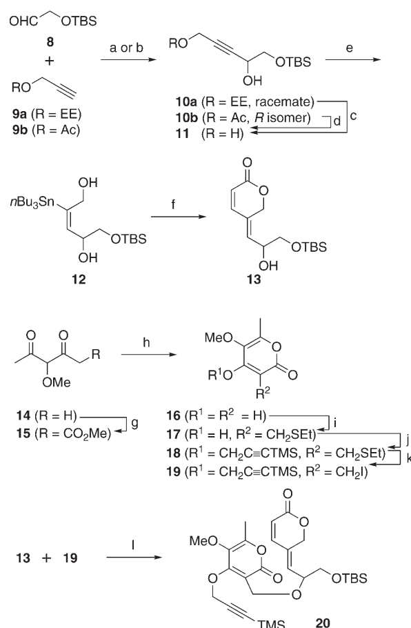
Scheme 4. Preparation of the dienophile, the pyrone, and their coupling. Reagents and conditions: a) n BuLi, THF, −78 °C, 94% (from 9a to 10a ); b) Zn(OTf) 2 , Et 3 N, (1 R ,2 R )-3-( tert -butyldimethylsilyloxy)-2- N,N -dimethylamino-1-( p -nitrophenyl)propan-1-ol, toluene, RT, 64% ( 9b → 10b ); c) PPTS, EtOH, RT, 66%; d) DIBALH, CH 2 Cl 2 , −78 °C, 87%; e) n Bu 3 SnH, [Pd(PPh 3 ) 4 ], THF, 0 °C; f) ( Z )-ICH=CHCO 2 Me, copper(I) thiophene-2-carboxylate, NMP, 0 °C→RT, 50% (2 steps); g) LDA, ClCO 2 Me, ether, −78→0 °C, 82%; h) DBU, C 6 H 6 , reflux; i) EtSH, (CH 2 O) m , CHCl 3 , reflux, 91% (2 steps); j) TMSC≡CCH 2 OTs, K 2 CO 3 , [18]crown-6, acetone, RT, 40%; k) MeI, C 6 H 6 , reflux, 87%; l) AgOTf, 4- A MS, 2,6-di- tert -butylpyridine, CH 2 Cl 2 , 0 °C→RT, 88%. DBU = 1,8-diazabicyclo[5.4.0]undec-7-ene, DIBALH = diisobutylaluminum hydride, LDA = lithium diisopropylamide, NMP = N -methylpyrrolidone, PPTS = pyridinium toluene- p -sulfonate, Tf = trifluoromethanesulfonyl, Ts = toluene- p -sulfonyl.
